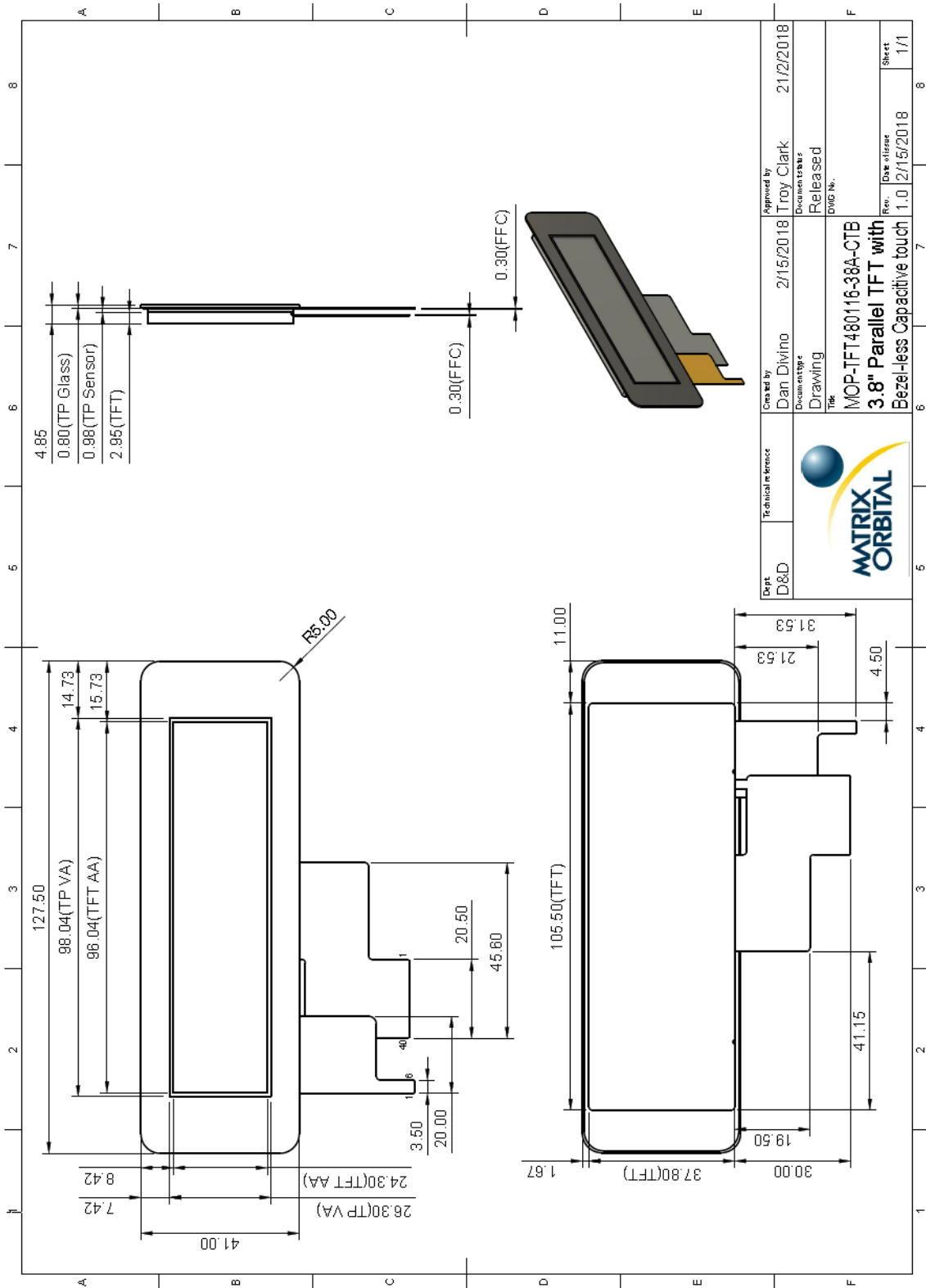
Figure 1: MOP-TFT480116-38A-BLH-CTB Drawing
