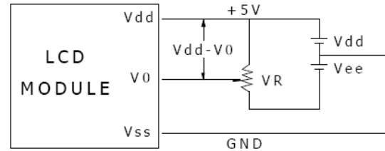
Figure 7: Display without Negative Voltage Output
