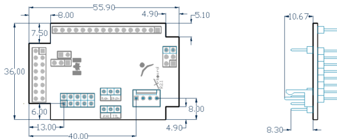
Figure 1: X-Board (S-Series)
