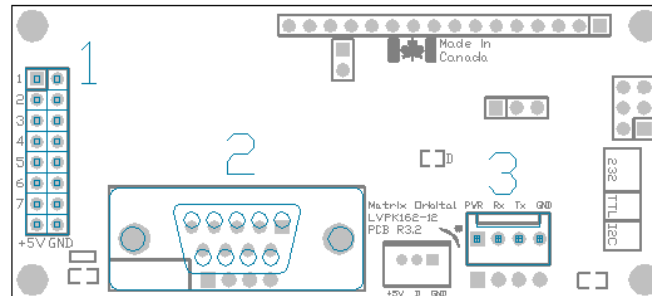
Figure 2: VK162-12 Header Locations
