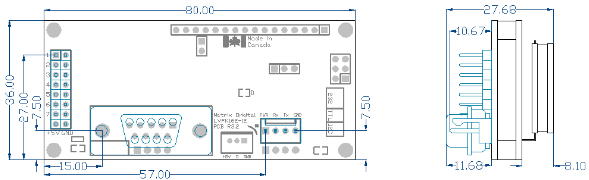
Figure 18: VK162-12 Dimensional Drawing
