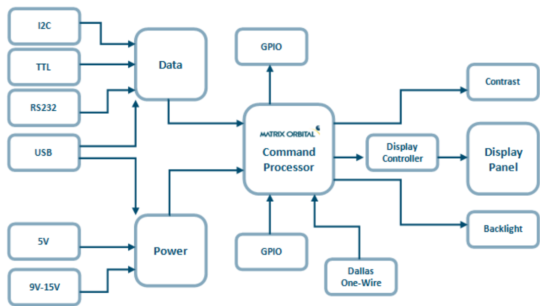
Figure 16: Functional Diagram
