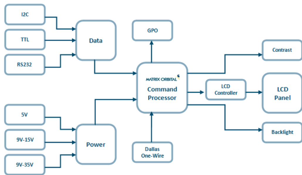
Figure 13: Functional Diagram
