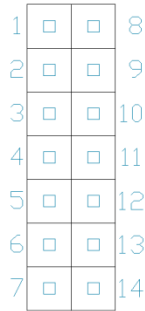
Figure 9: GPO Header
